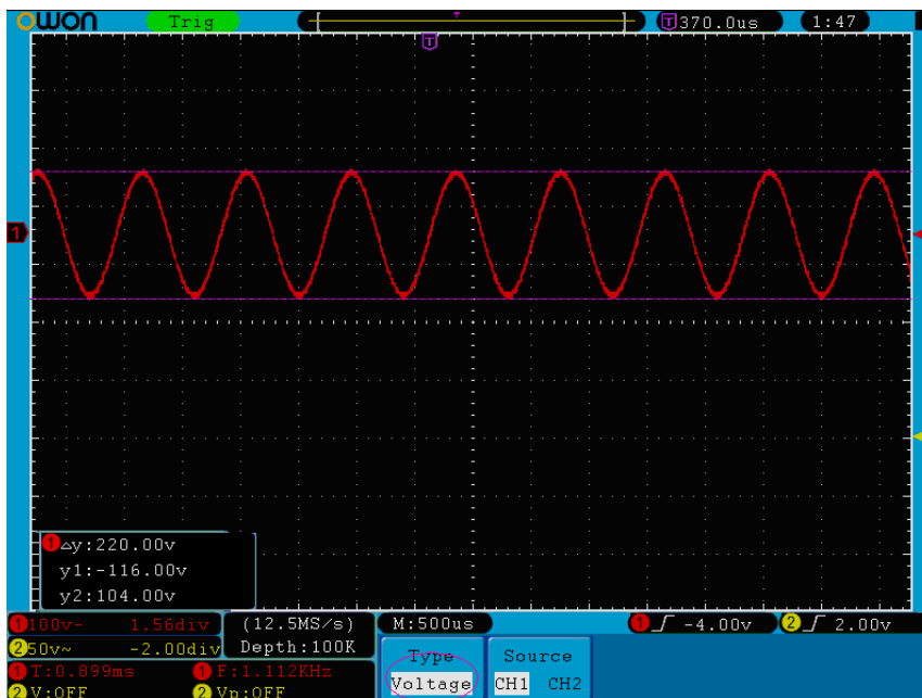
Figure 5-56 Waveform of Voltage Cursor Measurement
