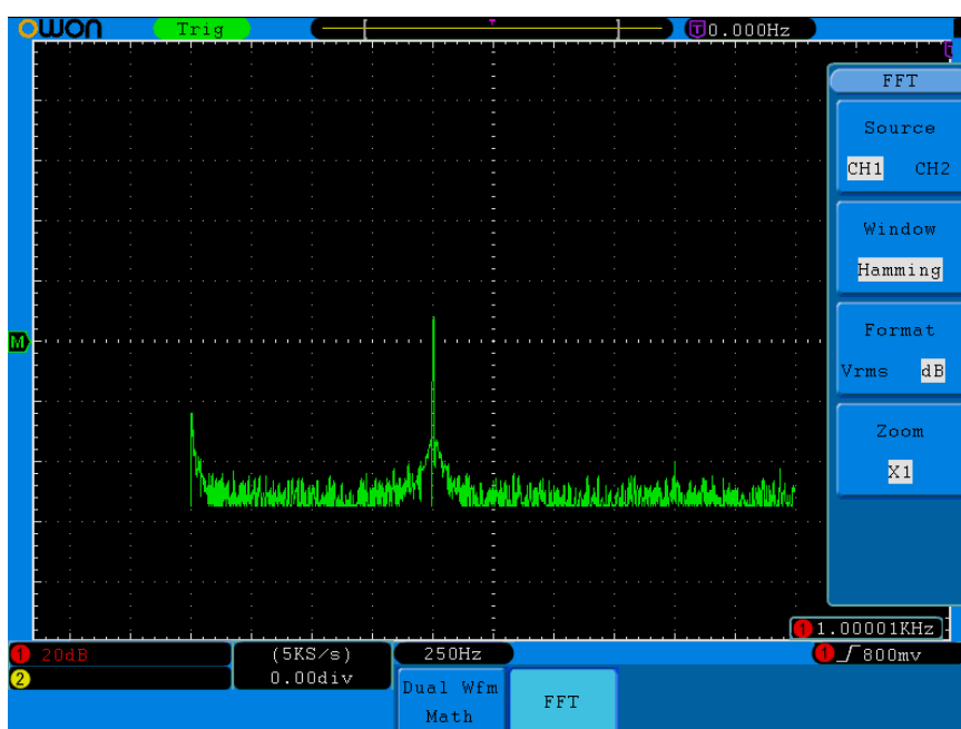
Figure 5-11 Hamming window
