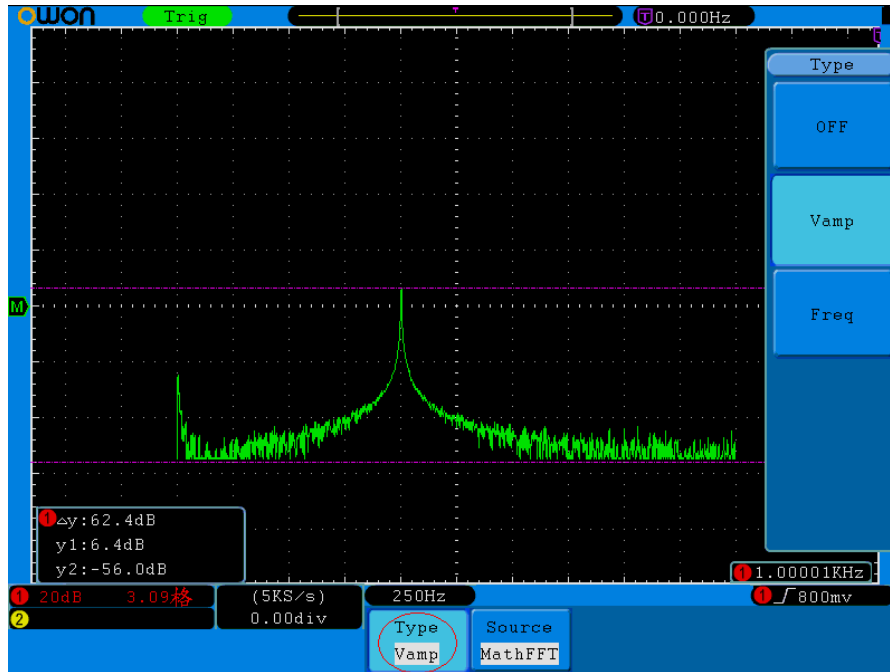
Figure 5-59 wave of Vamp cursor measurement
